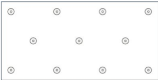
Figure 3 Fastener pattern (11 No. per board) Board size to 2.270 x 1.200 - 4.03 fixings / m 2
