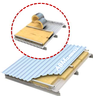
1. Double Skin Roof System
