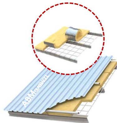
2. Single Skin Roof System
